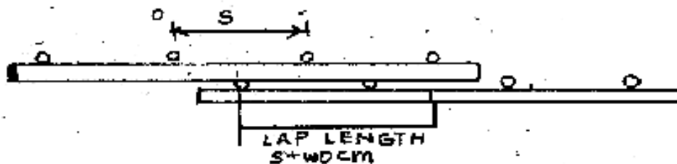
FIG -3 : LAP SPLICING OF WELDED WIRE FABRICS
