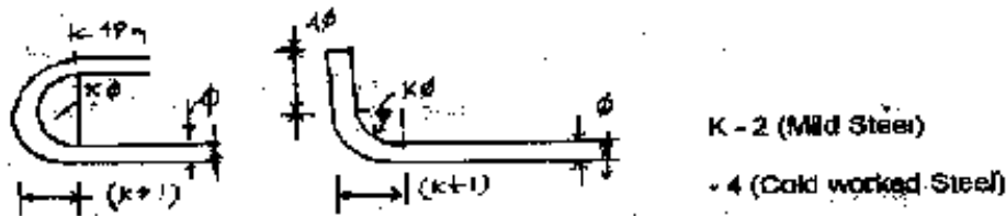
FIG-1: STANDARD HOOK AND BEND
